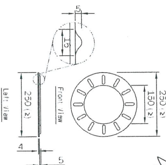
Stopper Board(9T)
