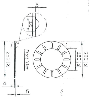
Stopper Board (9T)
