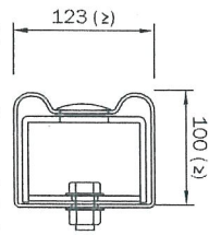
Sleeve Connect Detail View
