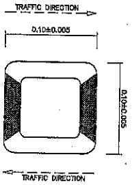
PLAN OF BI-DIRECTIONAL TYPE ROAD STUD TO SCALE NOT
