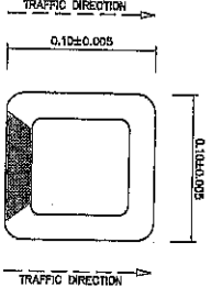
PLAN OF UNI-DIRECTIONAL TYPE ROAD STUD TO SCALE NOT
