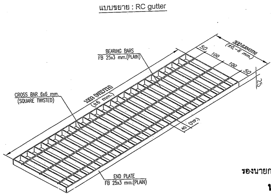
TYPICAL DETAIL TYPE GA 253/40 (PLAIN) Size 1003 mm.W x 300 mm.LB
