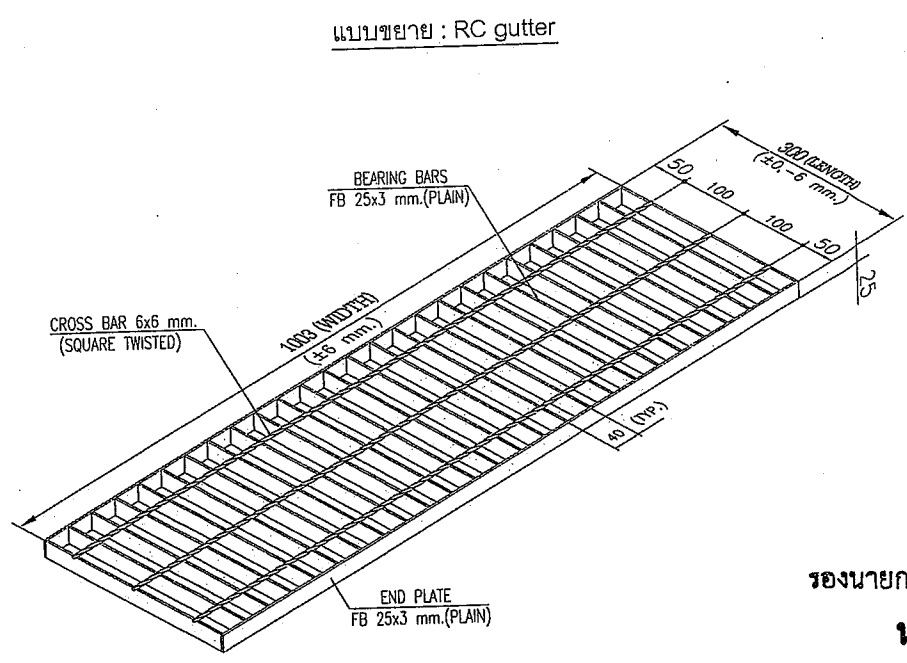
TYPICAL DETAIL TYPE GA 253/40 (PLAIN) Size 1003 mm.W x 300 mm.LB
